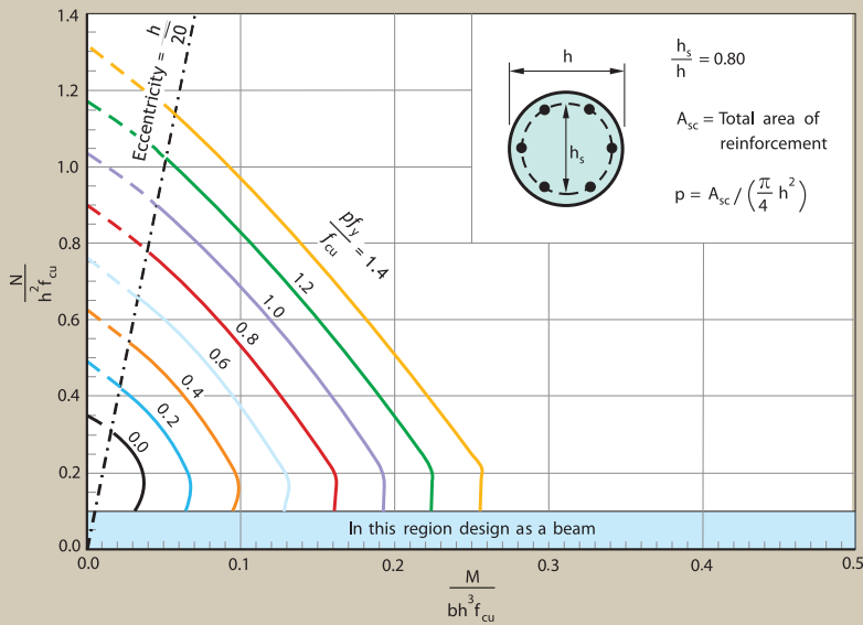
Column design chart for circular column h_s/h = 0.8
